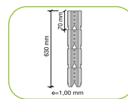
Cabides PF 61/T-45
